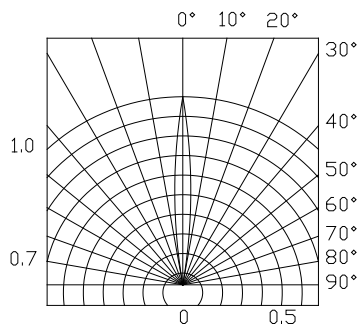
SPATIAL DISTRIBUTION
